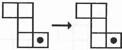
TRANSLATION
