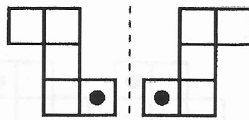
REFLECTION
